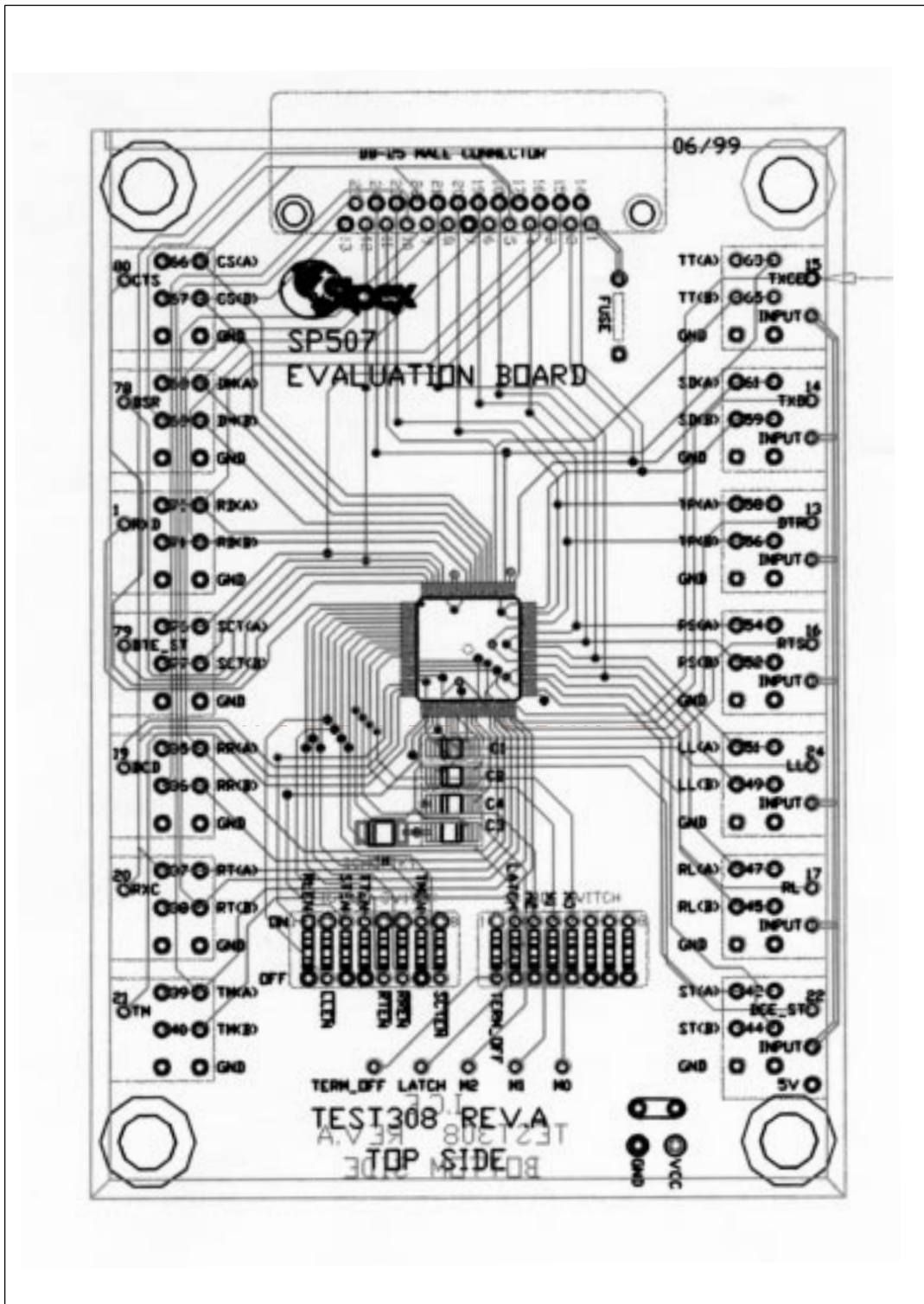
Figure 38. SP507 Evaluation Board Layout
