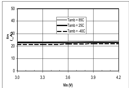
No Load Battery Current, V_{OUT} = 1.5\text{V}
