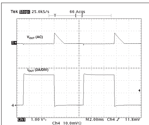
Figure 5. Load Transient ( V_{IN}=4V , V_O=3.3V , C_{OUT}=22\mu F , 10mA \sim 5A )
