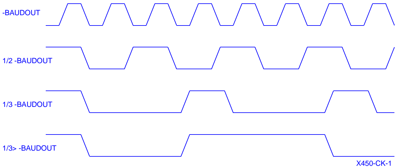
Clock timing
