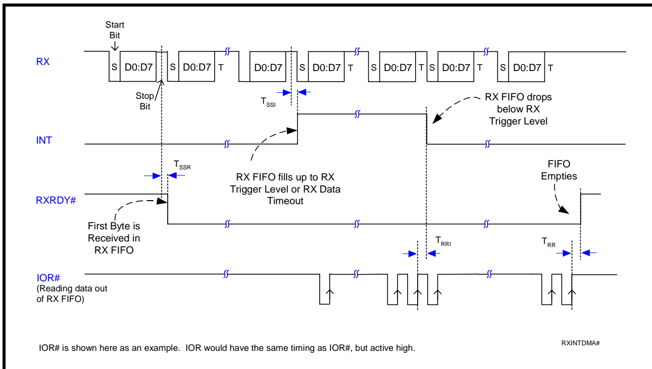
FIGURE 28. RECEIVE READY & INTERRUPT TIMING [FIFO Mode, DMA Disabled]
