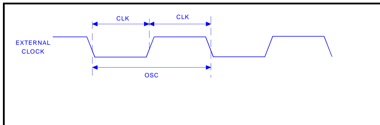
FIGURE 16. CLOCK TIMING
