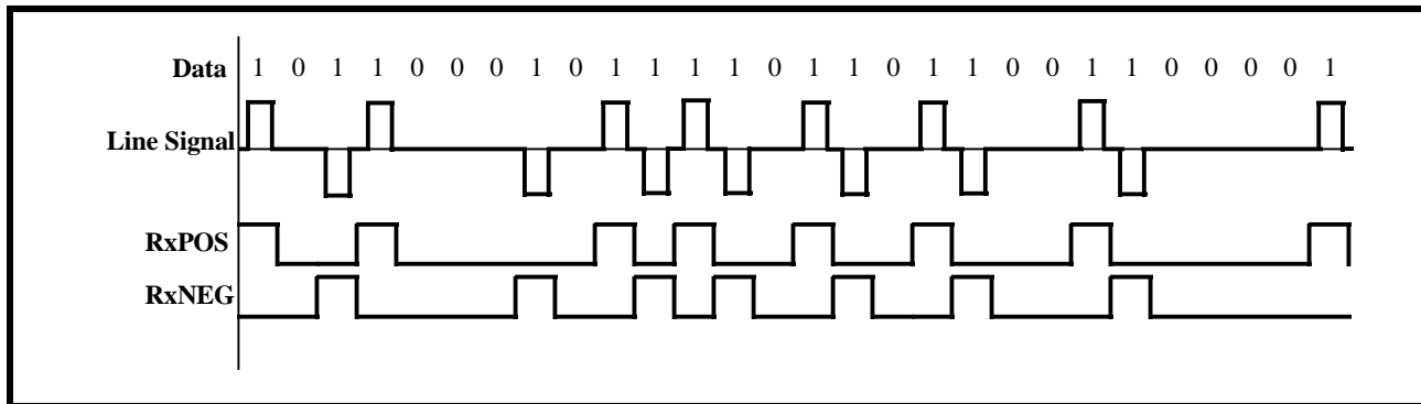
FIGURE 119. ILLUSTRATION OF AMI LINE CODE
