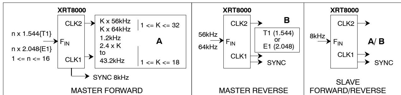
Figure 1. System Diagram
