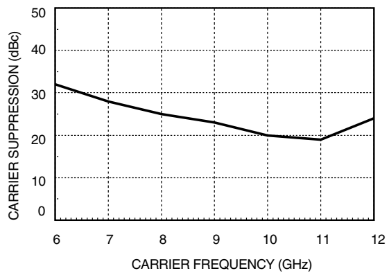
Carrier Suppression *
