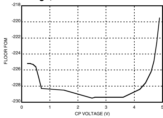
Figure 10. Floor FOM vs. CP Voltage, CP Current = 2.5mA
