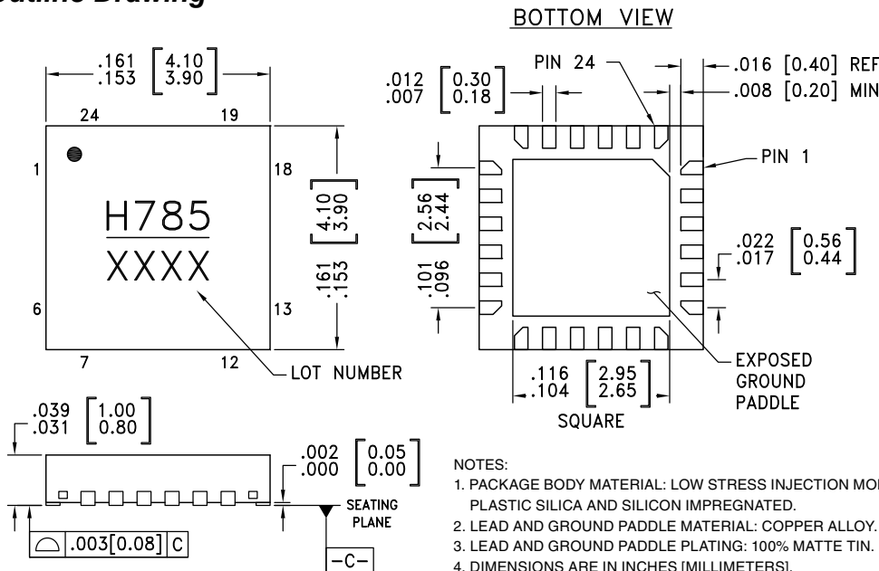
Outline Drawing
