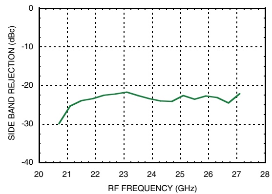
Sideband Rejection
