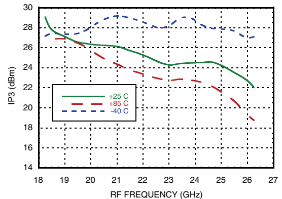
Output IP3, LSB vs. Temperature
