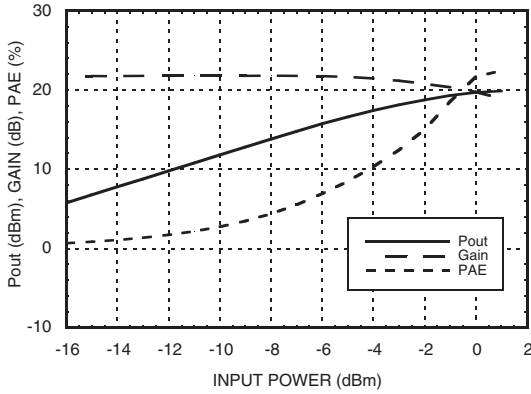
Power Compression @ 1700 MHz [1]
