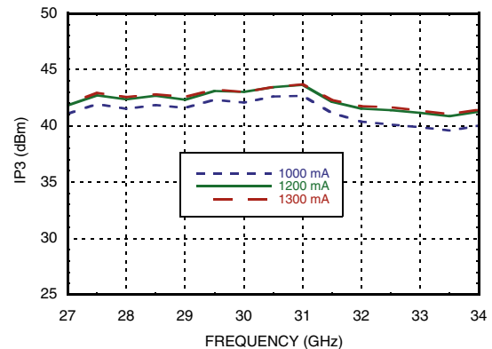
Output IP3 vs. Supply Current, Pout/Tone = +23 dBm
