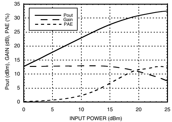
Power Compression @ 20 GHz
