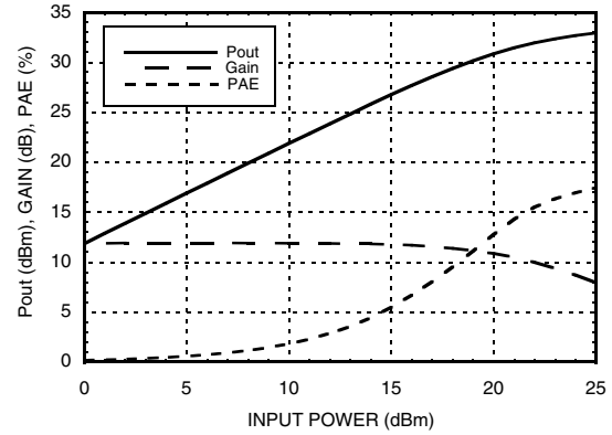
Power Compression @ 4 GHz
