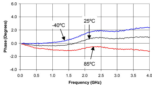
Phase - 8 dB Bit vs. Frequency Relative to Reference Loss State
