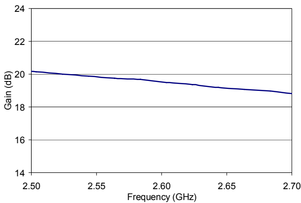
Gain, Vcctrl = 0V
