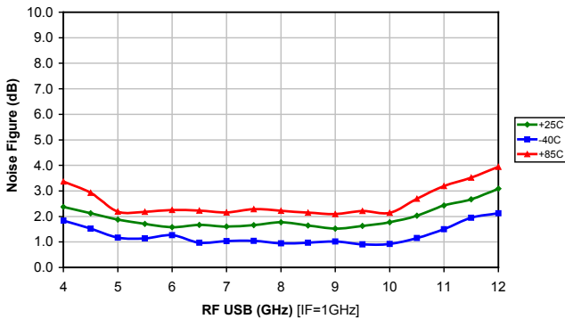
XR1011-QH: USB Noise Figure (dB) 4V @ 130mA, PLO=5dBm
