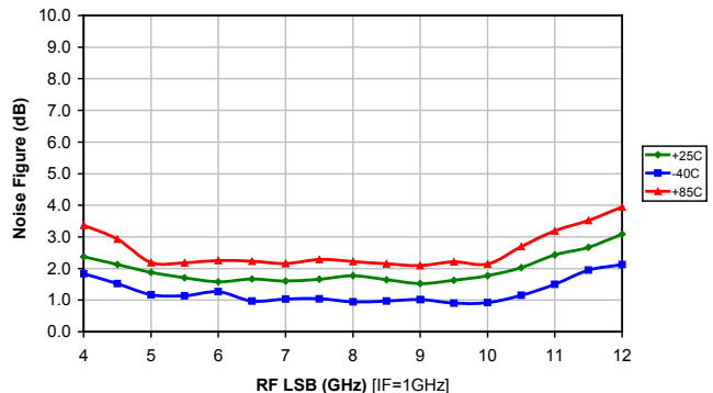
XR1011-QH: LSB Noise Figure (dB) 4V @ 130mA, PLO=5dBm
