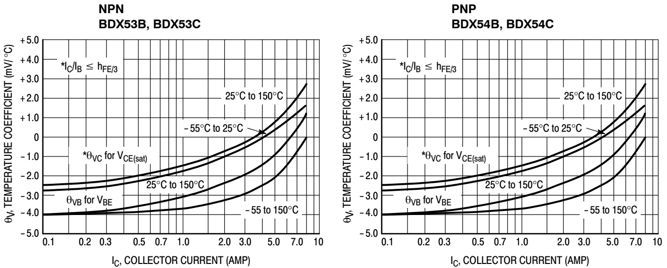
Figure 11. Temperature Coefficients
