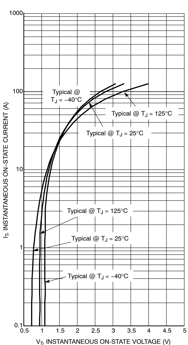
Figure 3. On-State Characteristics
