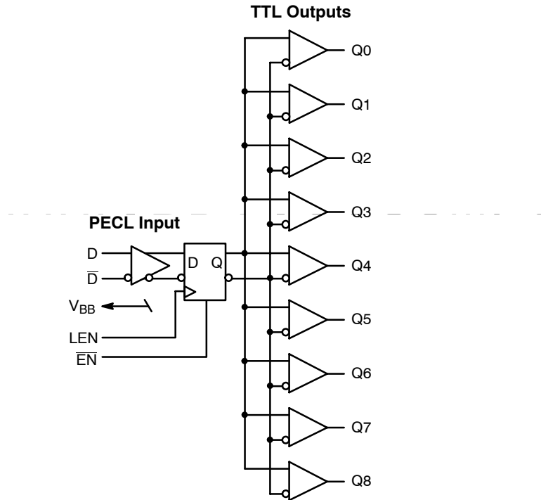
Figure 2. Logic Diagram
