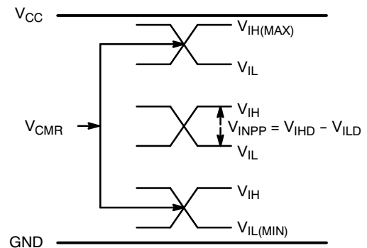
Figure 18. V_{CMR} Diagram
