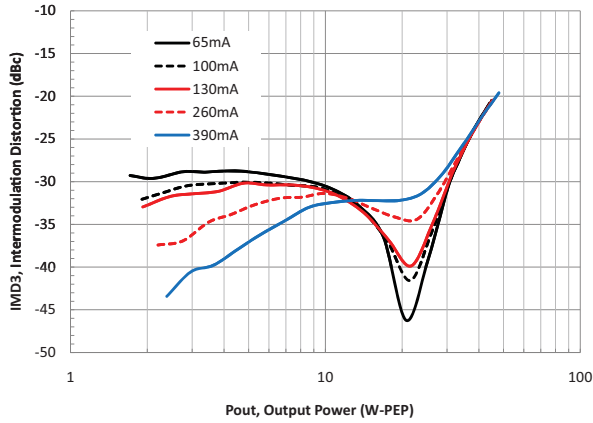
IMD3 vs. Pout (2-Tone 1MHz Separation, Vd = 48V, Idq varied, fc = 2140MHz)
