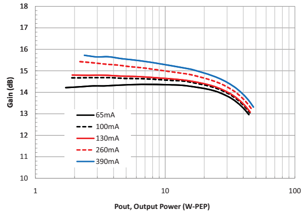
Gain vs. Pout (2-Tone 1MHz Separation, Vd = 48V, Idq varied, fc = 2140MHz)
