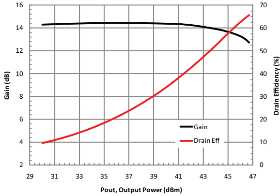
Gain/ Efficiency vs. Pout, f = 2140MHz (CW, Vd = 48V, Idq = 130mA)
