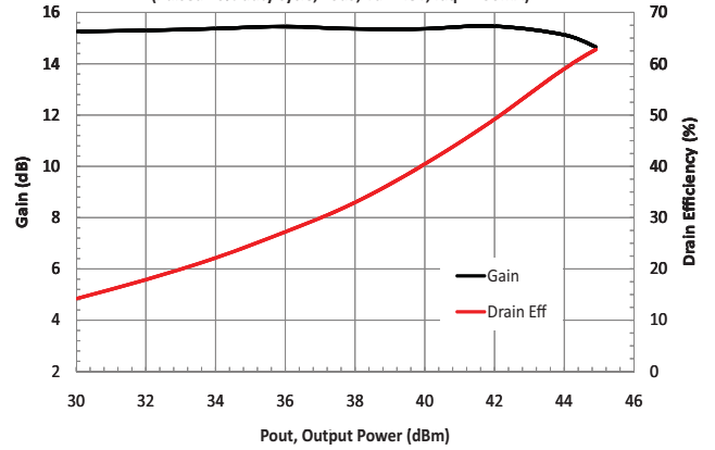
Gain/ Efficiency vs. Pout, f = 2140MHz (Pulsed 10% duty cycle, 10uS, Vd = 48V, Idq = 130mA)
