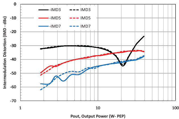
IMD vs. Output Power (Vd = 48V, Idq = 130mA, f1 = 2139.5MHz, f2 = 2140.5MHz)
