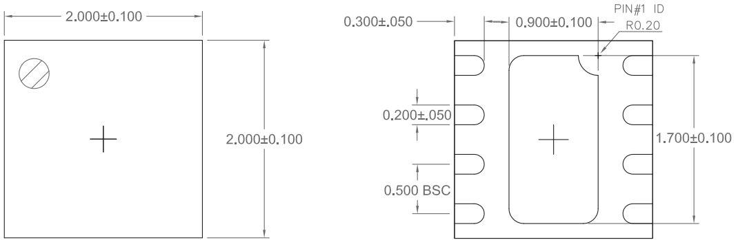
BOTTOM VIEW
