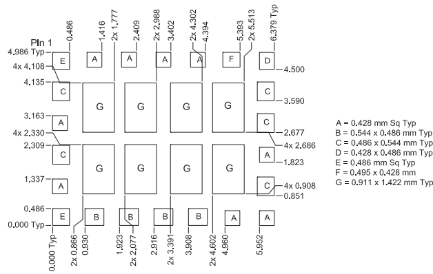
PCB STENCIL PATTERN
