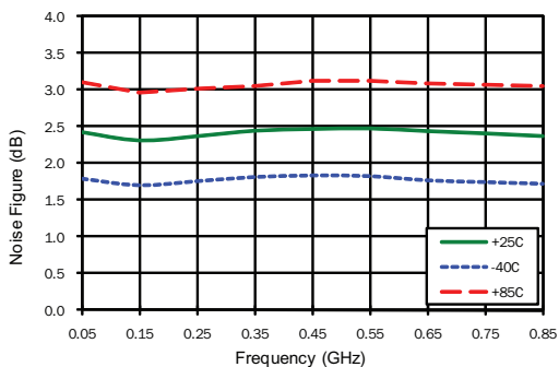
Noise Figure versus Frequency (Max Gain)
