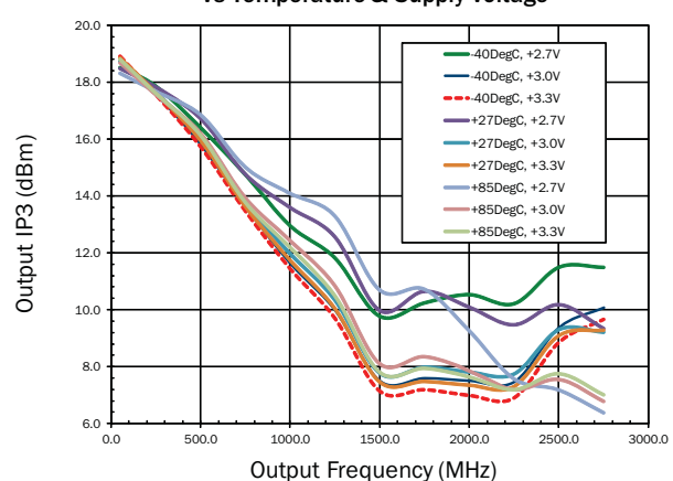
Modulator Output IP3 Vs Temperature & Supply Voltage
