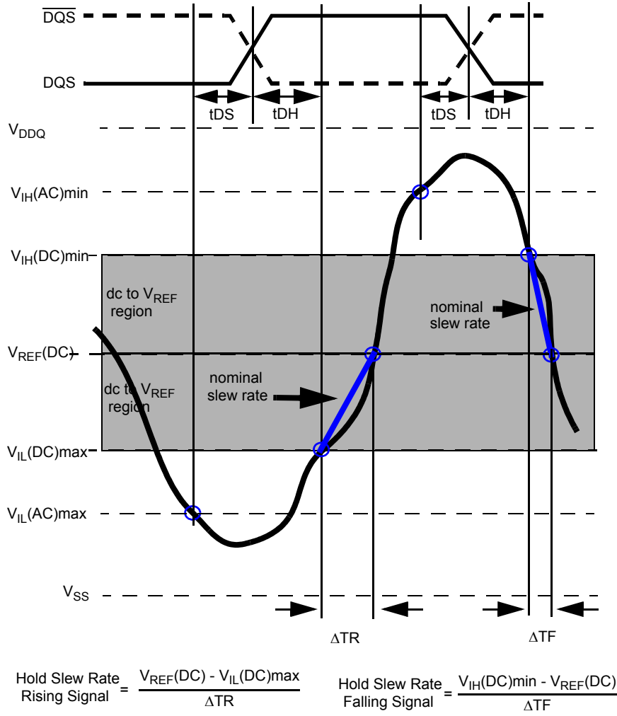
Figure 11. Illustration of nominal slew rate for tDH (differential DQS, QQS)
