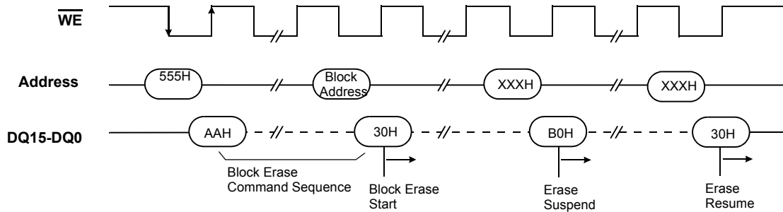
Figure 6: Erase Suspend / Resume Command Sequence
