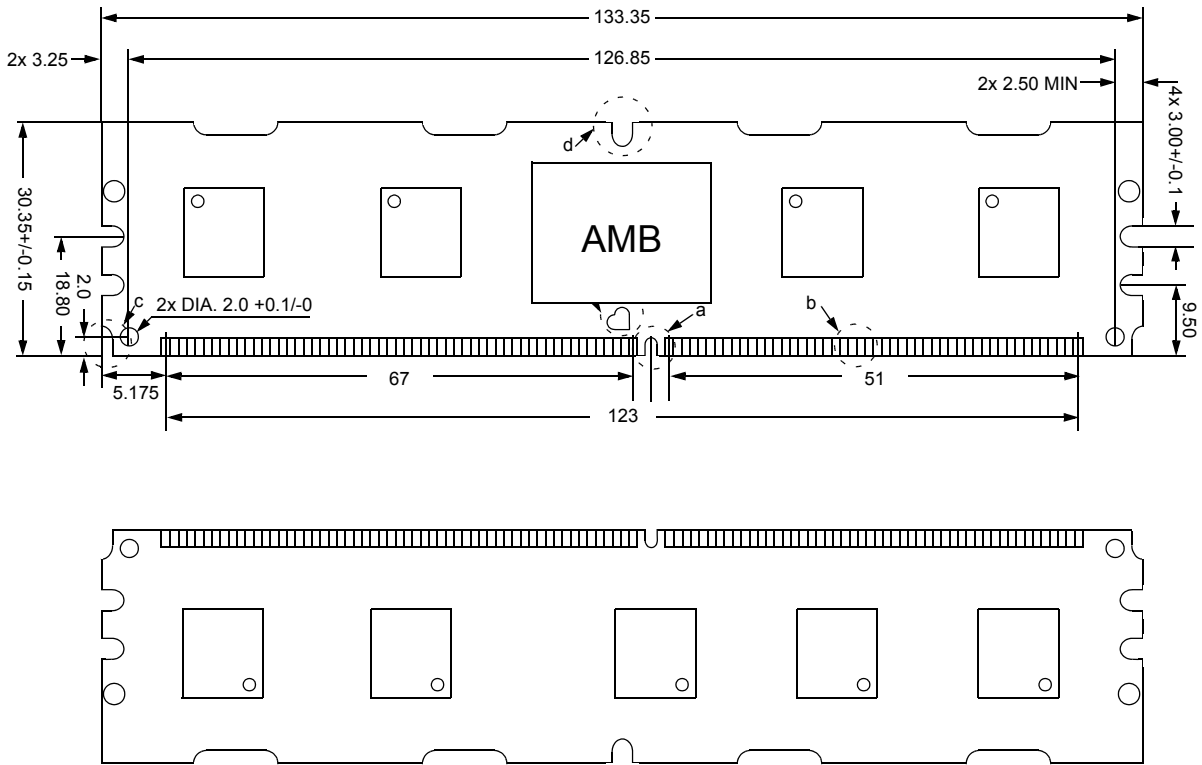
Figure 17 : FBDIMM Physical Dimension -1 (For PCB) : 64Mbx8 based 64Mx72 Module (1Rank) M395T6553CZ4
