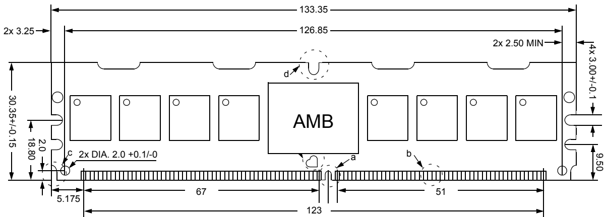
Figure 19 : FBDIMM Physical Dimension -1 (For PCB) : 64Mbx8 based 128Mx72 Module (2Rank) M395T2953CZ4
