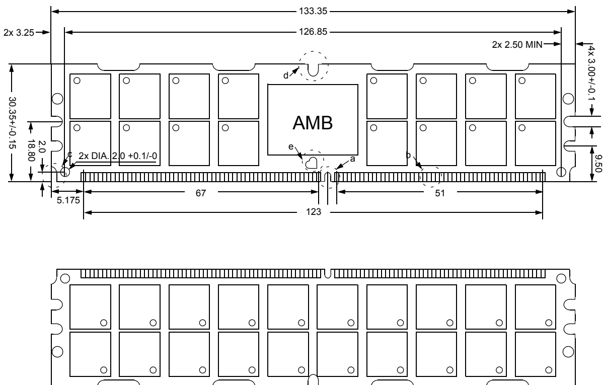
Figure 21 : FBDIMM Physical Dimension -1 (For PCB): 128Mbx4 based 256Mx72 Module (2Rank) M395T5750CZ4
