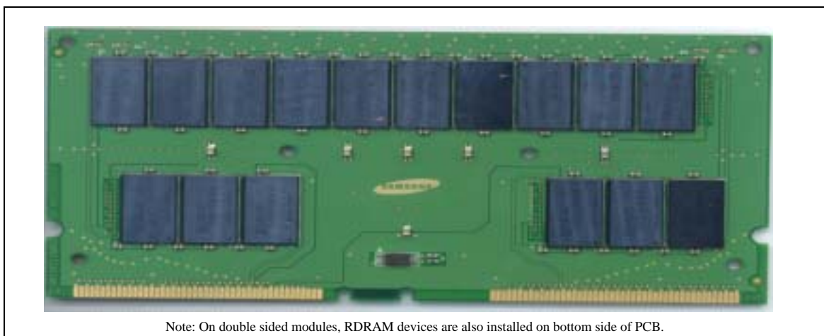
Figure 1: RIMM Module shown with heat spreader removed
