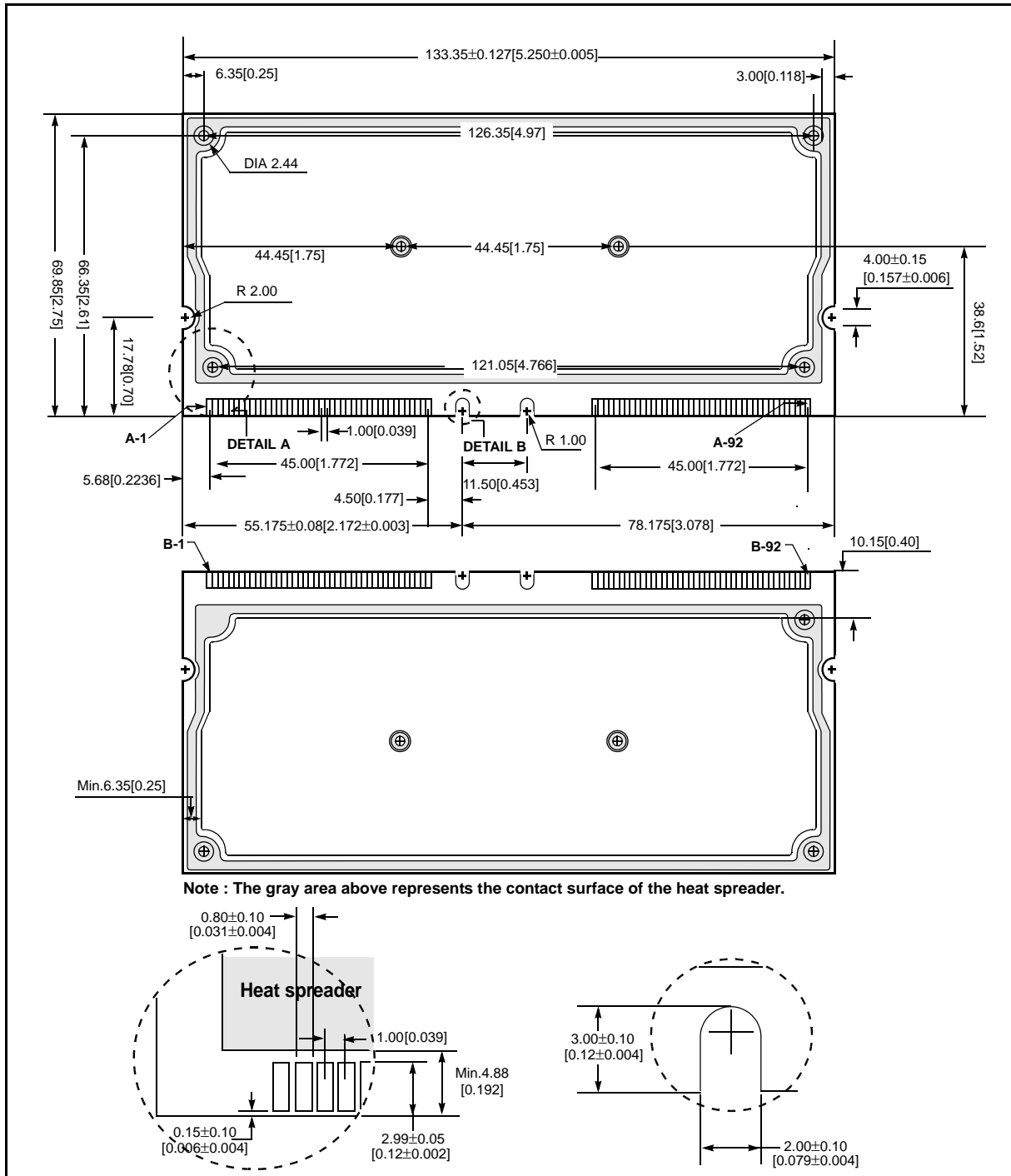
Figure 3: 32d RIMM Module PCB Physical Dimensions
