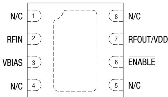
Figure 2. SKY67002-396LF Pinout – 8-Pin DFN (Top View)
