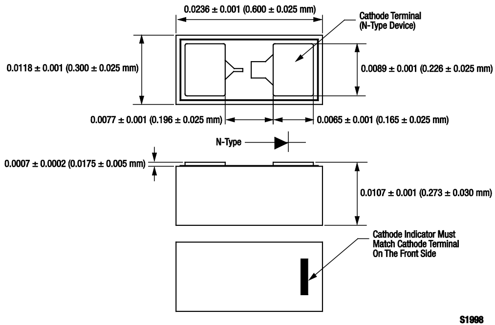
Figure 11. SMS7621-060 Package Dimension Drawing
