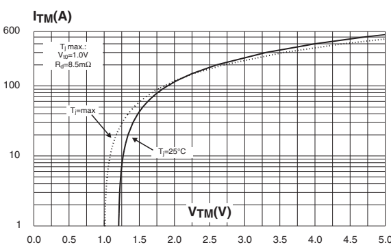
Figure 7: On-state characteristics (maximum values)
