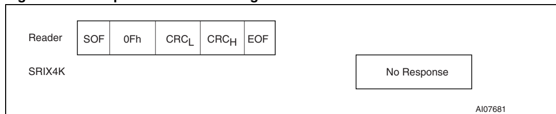
Figure 38. Completion frame exchange between reader and SRIX4K
