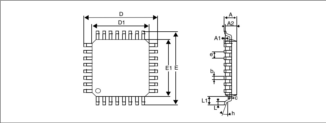
Figure 88. 32-pin low profile quad flat package outline
