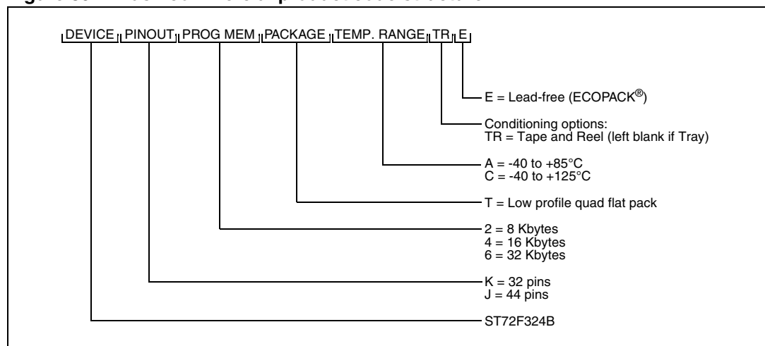
Figure 89. Flash commercial product code structure
