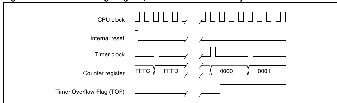
Figure 37. Counter timing diagram, internal clock divided by 4
