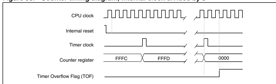
Figure 38. Counter timing diagram, internal clock divided by 8
