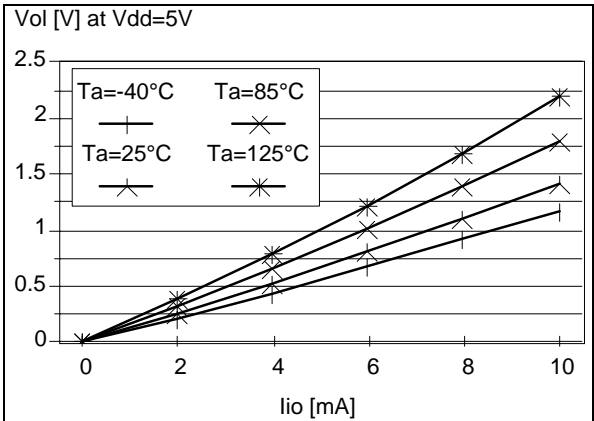
Figure 84. Typical V_{OL} at V_{DD}=5V (high-sink)
