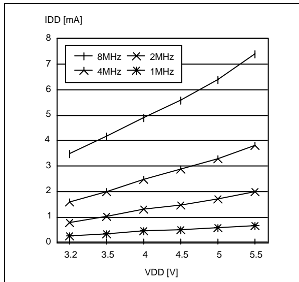
Figure 62. Typical I_{DD} in RUN vs. f_{CPU}
