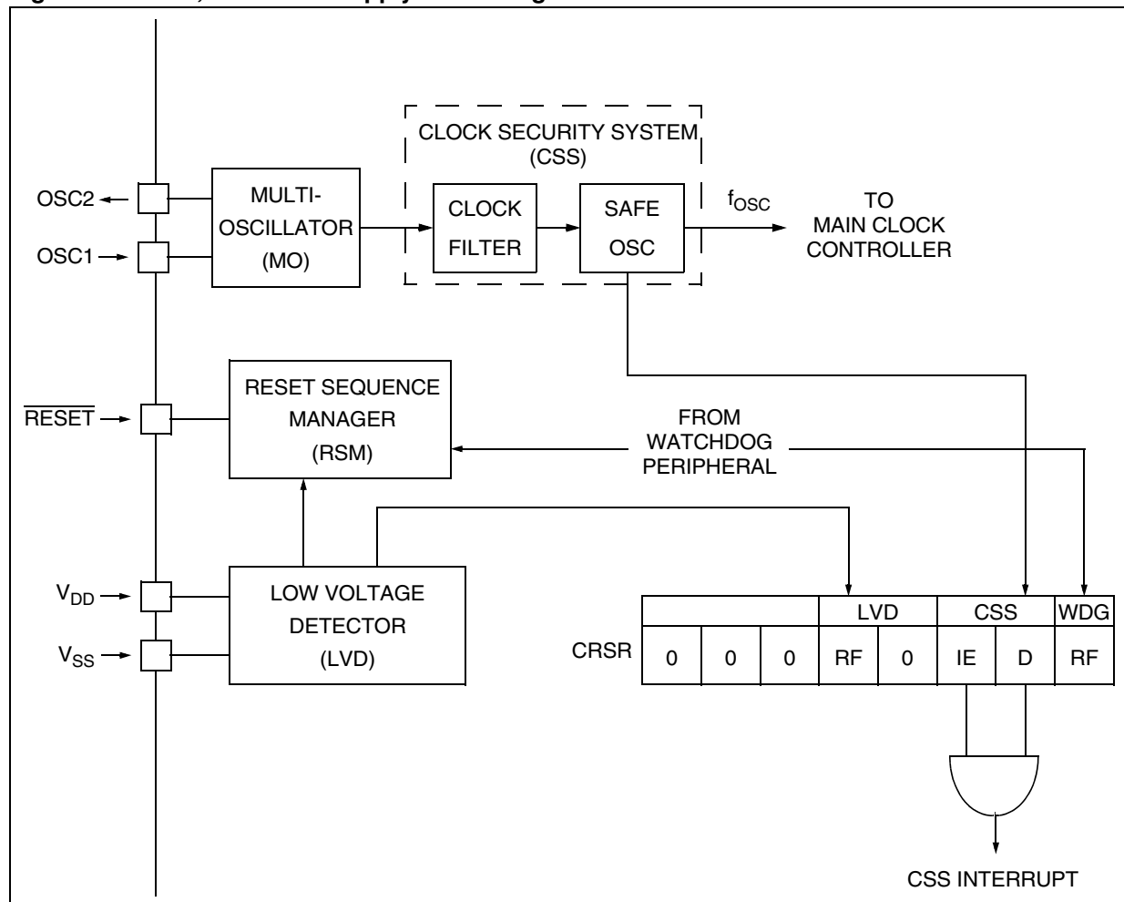
Figure 11. Clock, Reset and Supply Block Diagram
