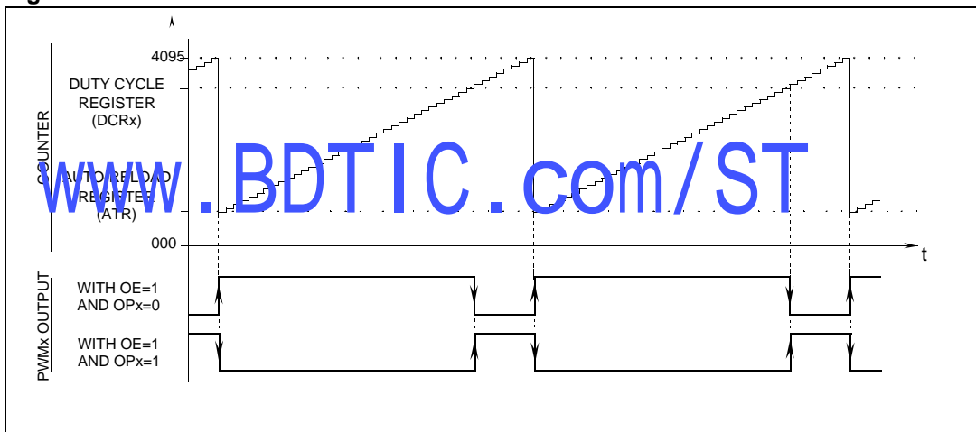
Figure 38. PWM function
