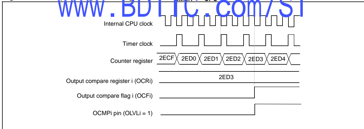
Figure 63. Output compare timing diagram, f_{IMPR} = f_{CPU}/2
