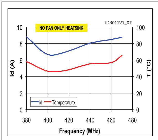
Figure 9. Drain current and temperature record on PCB surface
