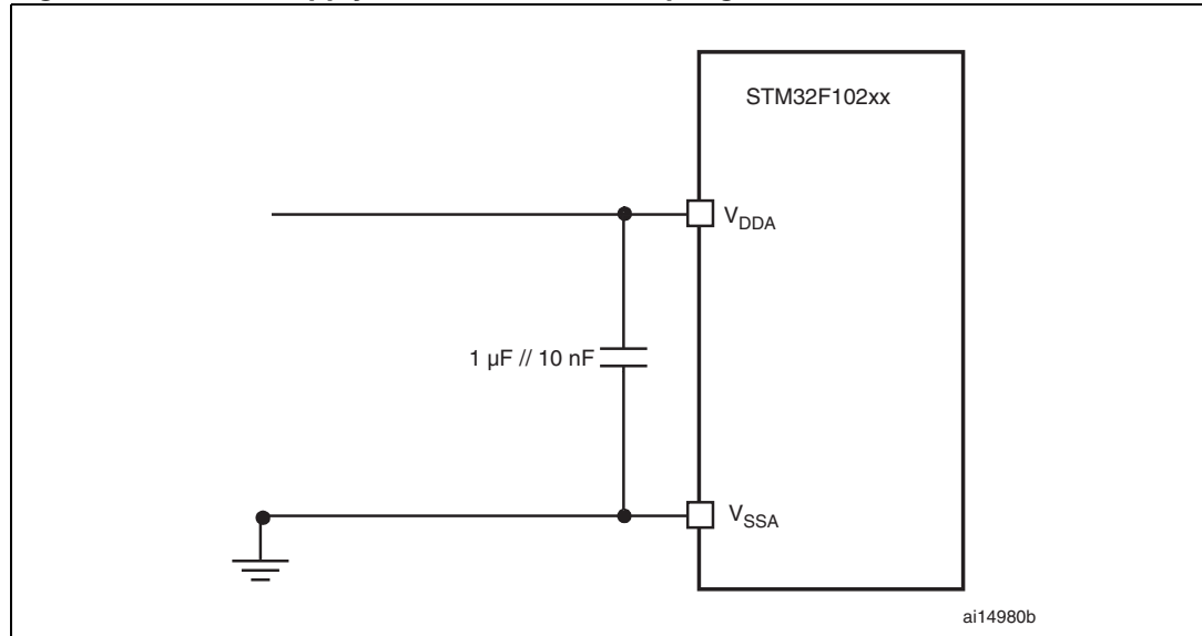
Figure 28. Power supply and reference decoupling
