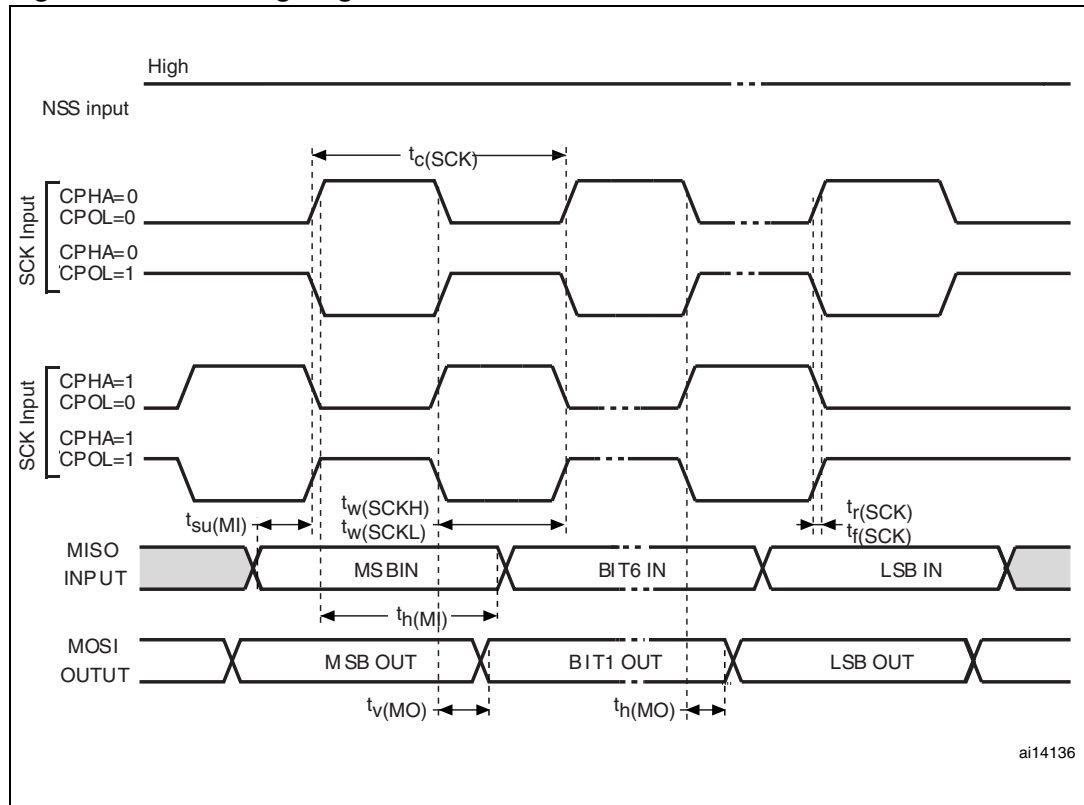
Figure 24. SPI timing diagram - master mode (1)
