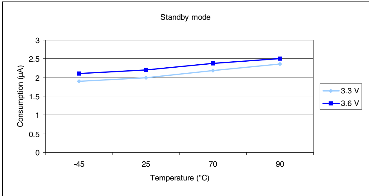
Figure 14. Typical current consumption in Standby mode versus temperature at V_{DD} = 3.3\text{ V} and 3.6\text{ V}
