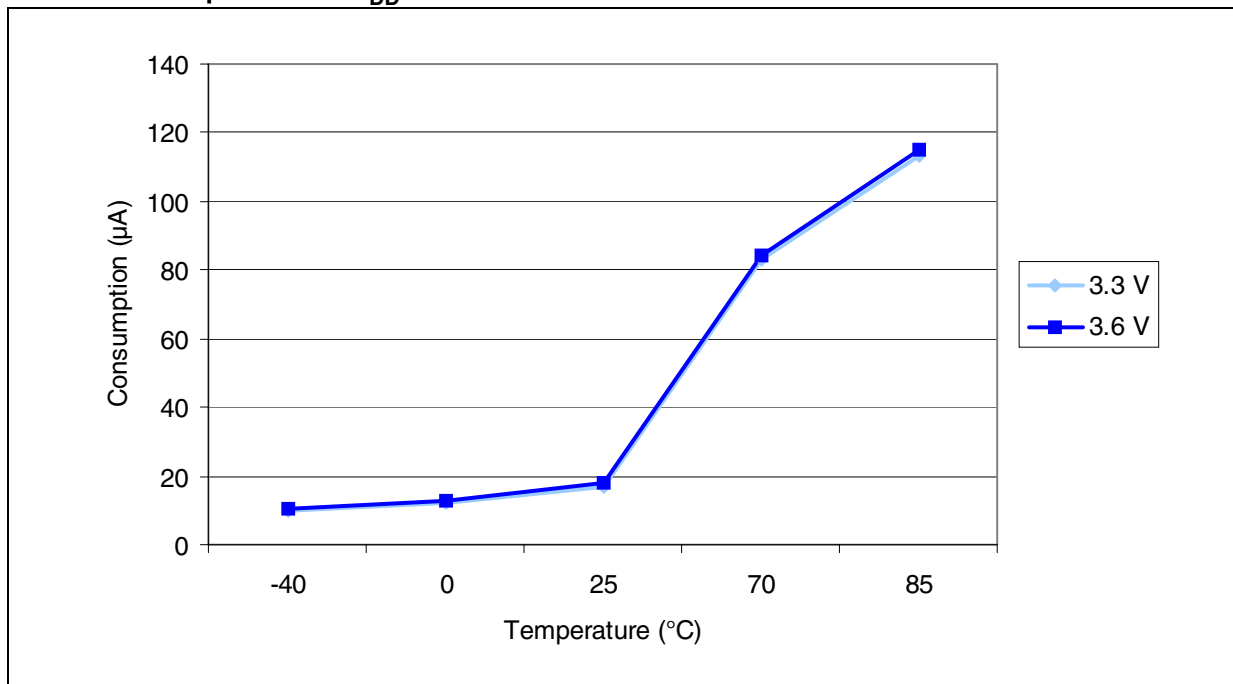
Figure 13. Typical current consumption in Stop mode with regulator in Low-power mode versus temperature at V_{DD} = 3.3\text{ V} and 3.6\text{ V}
