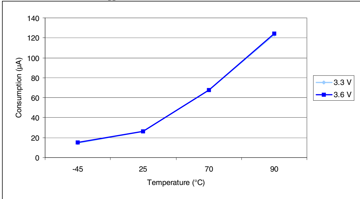
Figure 12. Typical current consumption in Stop mode with regulator in Run mode versus temperature at V_{DD} = 3.3\text{ V} and 3.6\text{ V}
