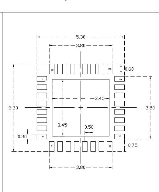
Figure 38. UFQFPN32 recommended footprint (1)(4)
