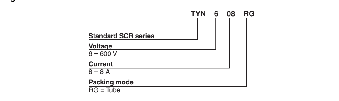
Figure 17. TYNx08 series
