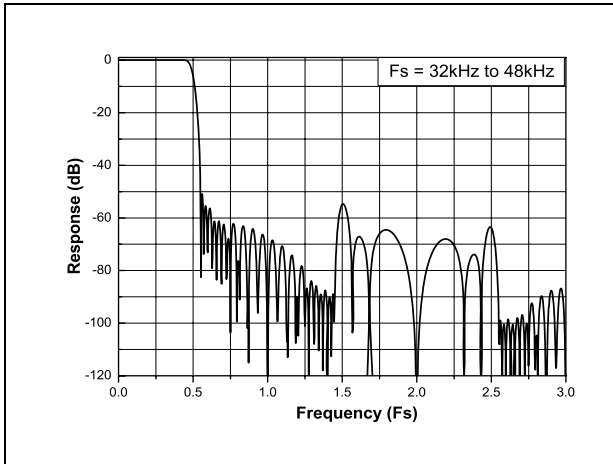
Figure 4. DAC digital filter frequency response from 32 to 48 kHz
