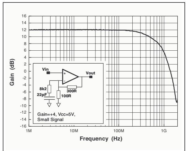
Figure 6. Compensation, gain=+4
