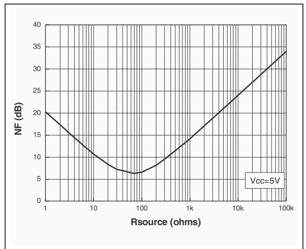
Figure 12. Noise figure
