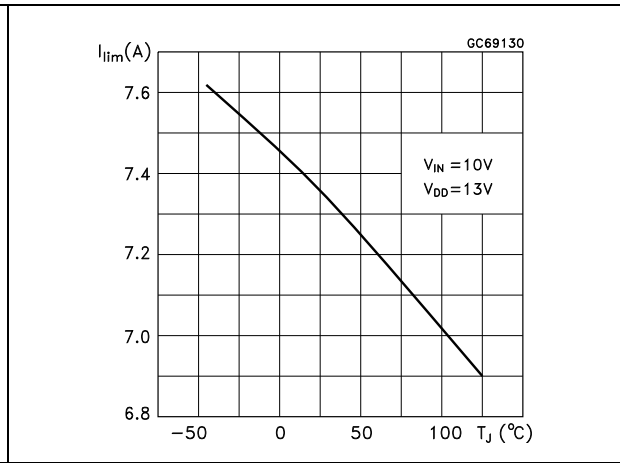
Figure 24. Step response current limit
