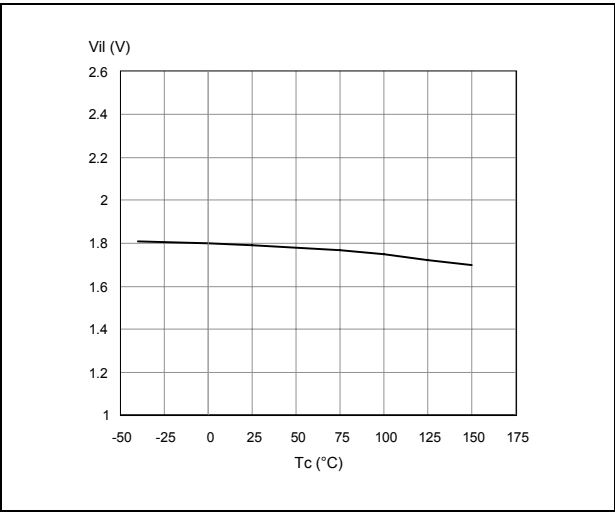
Figure 18. Input low-level
