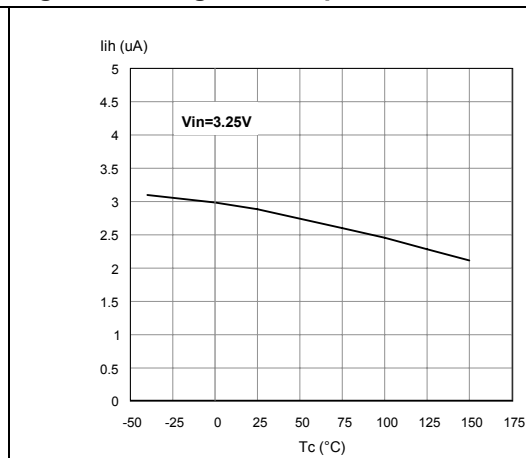
Figure 8. High-level input current
