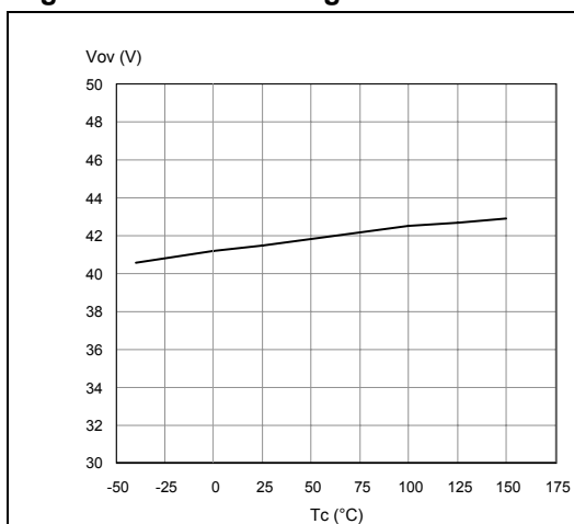
Figure 11. Over-voltage shutdown
