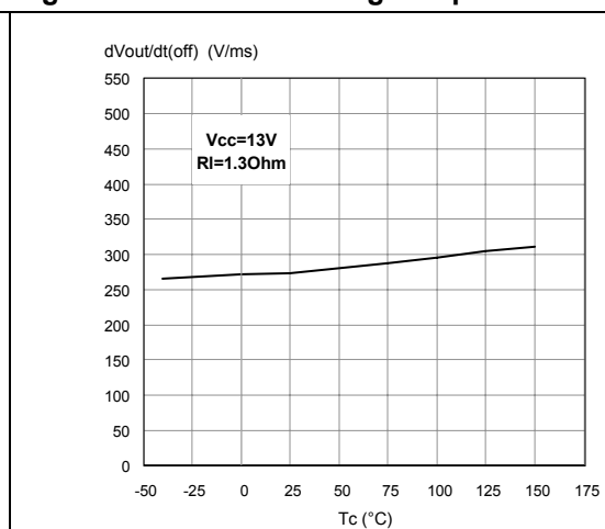
Figure 12. Turn-off voltage slope
