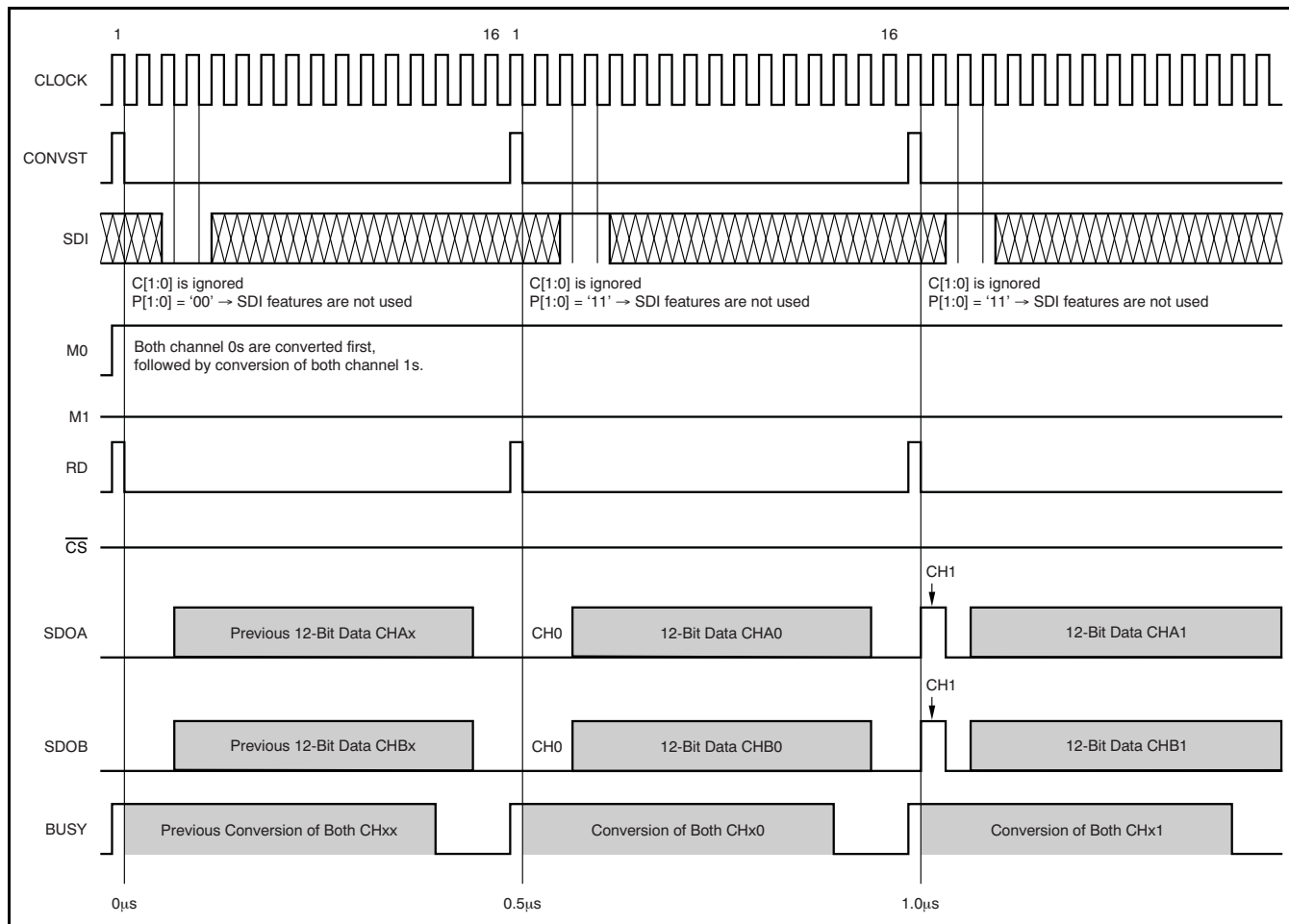
Figure 35. Mode III Timing Diagram (M0 = 1; M1 = 0)
