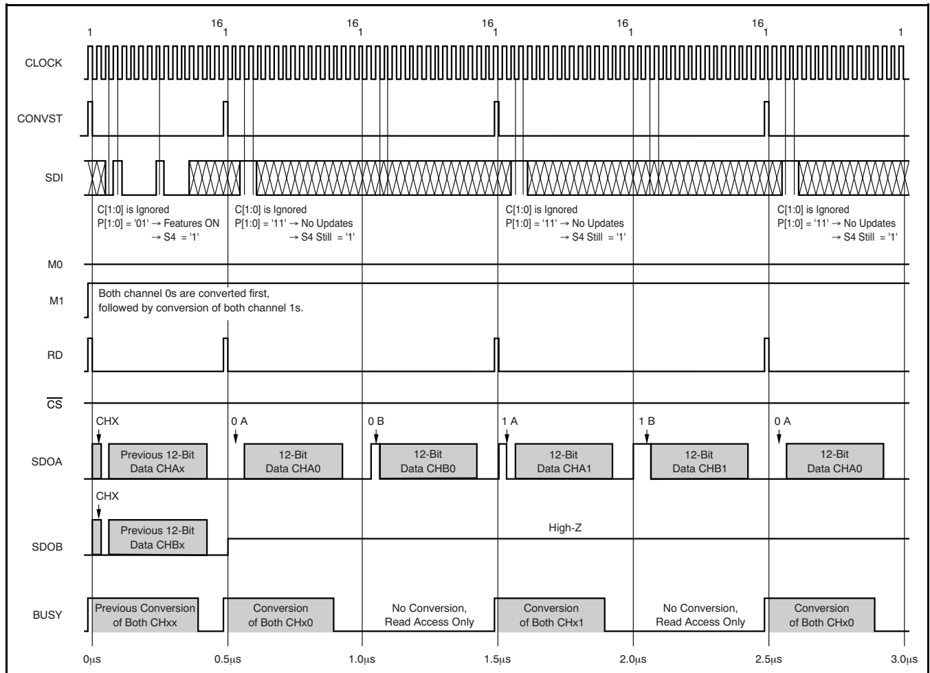
Figure 38. Special Mode IV Timing Diagram (M0 = 1; M1 = 1; S4 = 1)
