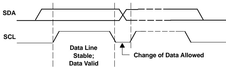
Figure 42. Bit Transfer on the I 2 C Bus
