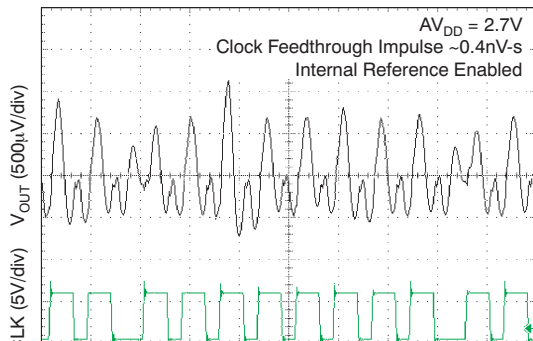
CLOCK FEEDTHROUGH 2.7V, 2MHz, MIDSCALE
