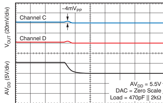
POWER-OFF GLITCH
