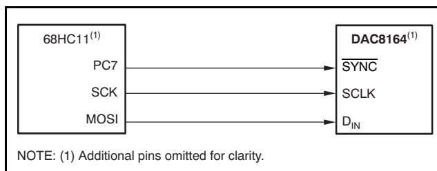
Figure 103. DAC8164 to 68HC11 Interface
